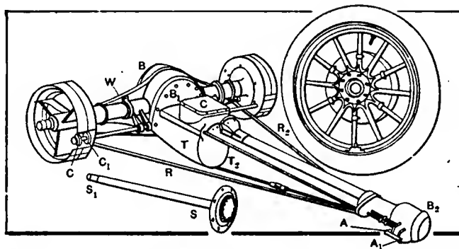
Fig. 12—Rear axle transmission unit, with wheels removed and showing the internal expanding brakes
